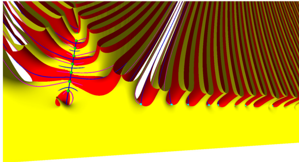
Fig. 3. \Re\zeta(s) and \Im\zeta(s) surfaces for (\sigma, t) \in (-40, 10) \times (-20, 100) .
