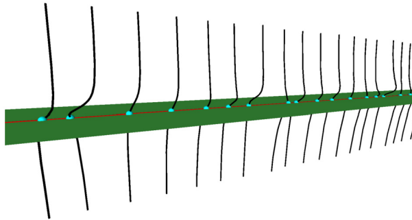
Fig. 7. 3D curves corresponding the intersections of \Re\zeta(s) and \Im\zeta(s) surfaces in the critical strip.
