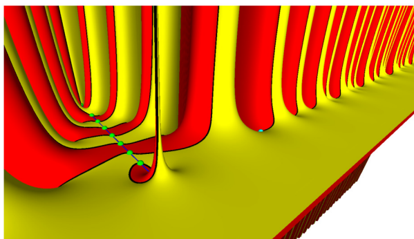
Fig. 5. \Re\zeta(s) and \Im\zeta(s) surfaces for (\sigma, t) \in (-40, 10) \times (-20, 100) .
