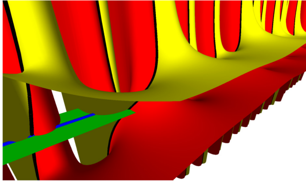
Fig. 8. \Re f(s, 3/4) and \Im f(s, 3/4) surfaces for (\sigma, t) \in (-1, 2) \times (1.65, 1.95) .
