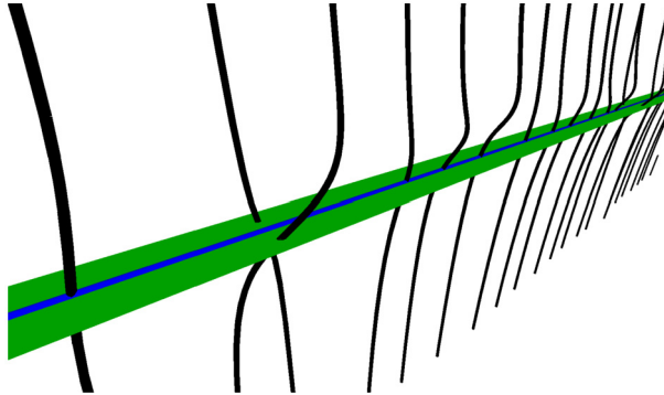
Fig. 9. 3D curves corresponding the intersections of \Re f(s, 3/4) and \Im f(s, 3/4) surfaces in the critical strip.
