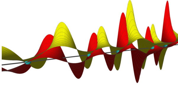
Fig. 1. Zeroes, \Re\zeta(s) and \Im\zeta(s) surfaces for (\sigma, t) \in (-1/2, 3/2) \times (10, 35) .
