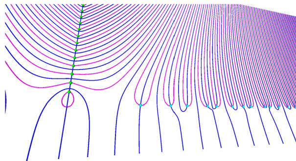
Fig. 4. 2D curves corresponding the intersections of \Re\zeta(s) and \Im\zeta(s) surfaces with the complex plane, (\sigma, t) \in (-40, 10) \times (-20, 100) .
