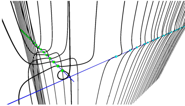
Fig. 6. 3D curves corresponding the intersections of \Re\zeta(s) and \Im\zeta(s) surfaces for (\sigma, t) \in (-40, 10) \times (-20, 100) .
