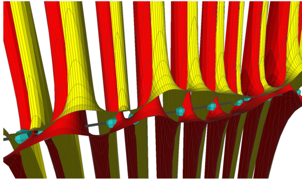
Fig. 2. Zeroes, \Re\zeta(s) and \Im\zeta(s) surfaces for (\sigma, t) \in (-1/2, 3/2) \times (10, 35) .
