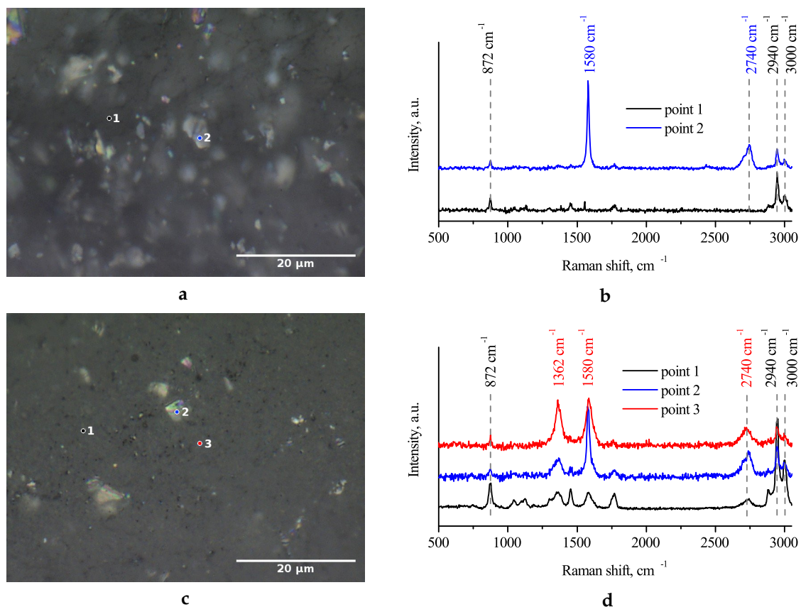
Figure 1. Optical microscopy image (a) and Raman spectra (b) of PLA composite containing 1.5% GNP. Due to the neat PLA transparency, it is possible to see GNPs under the surface of a composite. Optical microscopy image (c) and Raman spectra (d) of PLA composite containing the mixture of 3% GNP and 3% MWCNT. Raman spectrum collected at point 2 combines the characteristic peaks of PLA, GNPs, and MWCNTs.
