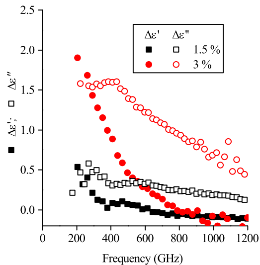
Figure 7. Impacts ( \Delta\epsilon_{cp} ) of cross-filler percolation to the dielectric permittivity of composites containing 1.5% MWCNT + 1.5 % GNP and 3% MWCNT + 3% GNP (referred to as 1.5% and 3%, respectively). Both real and imaginary parts behave typically for a percolated composite.
