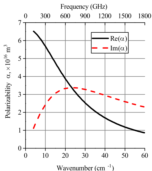
Figure 4. Frequency dispersion of the longitudinal polarizability calculated for oblate ellipsoid with a = b = 5 \mu\text{m} , c = 25 \text{ nm} (i.e., \text{AR} = 200 ), \sigma = 10,000 \text{ S/m} and \epsilon_m = 2.5 - 0.1i .
