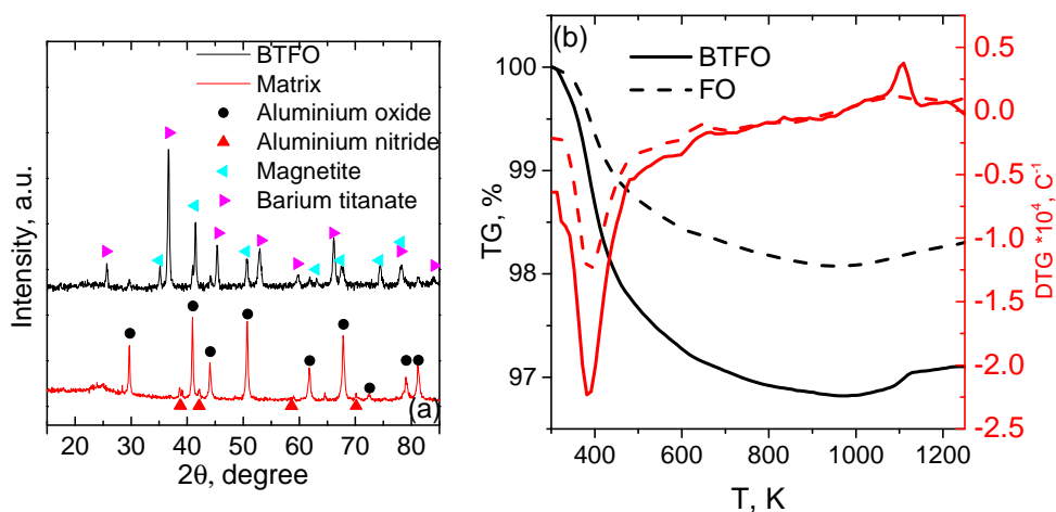
Figure 2. X-ray diffraction pattern of the BTFO and phosphate matrix (a). Thermogravimetric analysis of the BTFO and FO samples (b).
