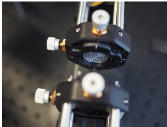
Figure 4. Photo of high-resistivity silicon-based Bessel zone plate placed in the optical mount. The diffractive optical element is prepared by the laser ablation technology. More details on fabrication technology and the zone plate design can be found in Ref. [213]. Photo: courtesy of Domas Jokubauskis.
